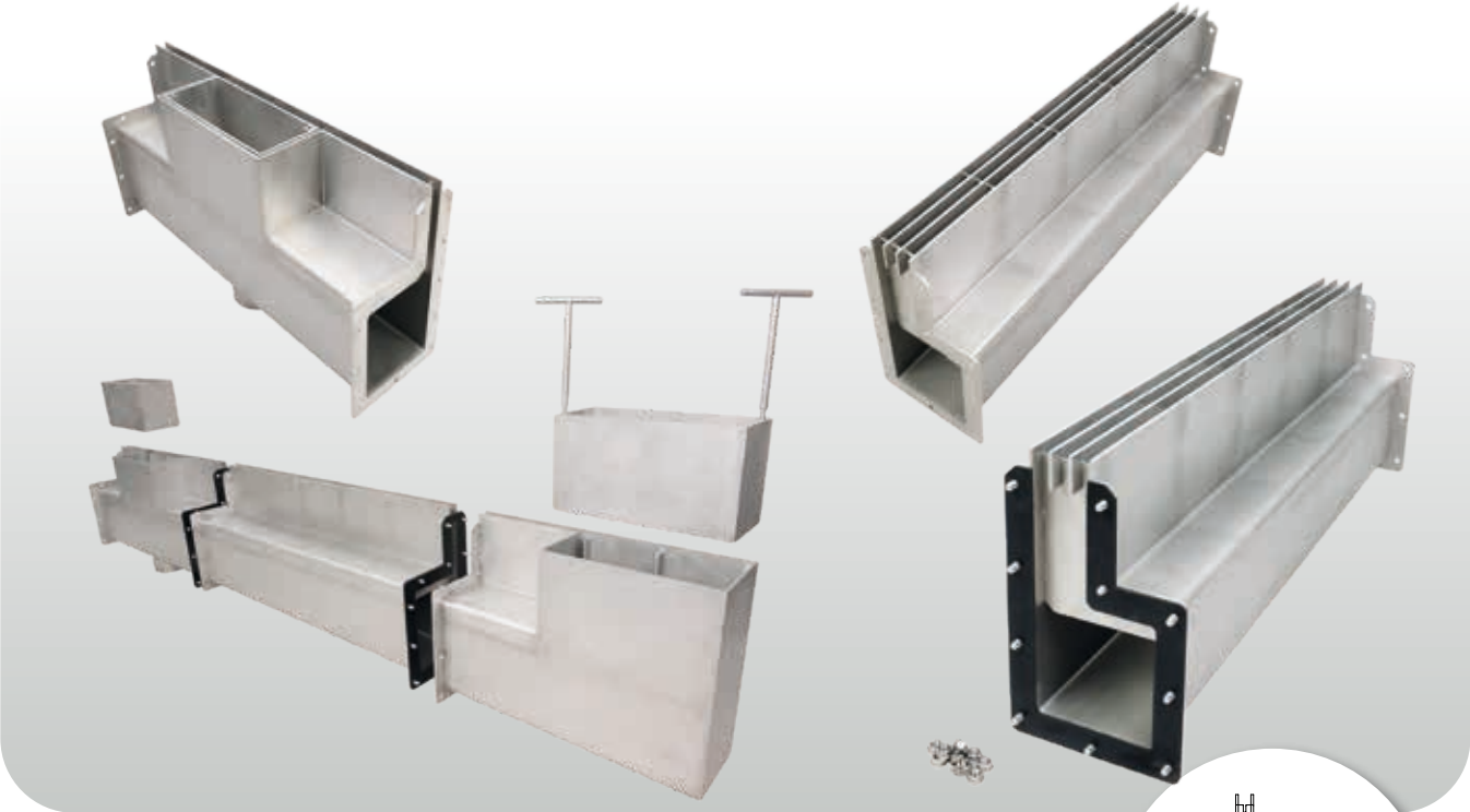
Lamina | slotted channels for fountains (1 chamber) made of stainless steel (V2A) 3.0 mm Standard length: 1,000 mm
